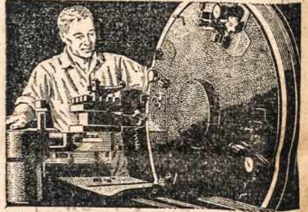
A horizontal engine lathe at Willow Run carrying Ford-designed equipment turns a gun-turret track for a B-24 Liberator. This machine saves time and holds the work to 1/10,000 of an inch.
