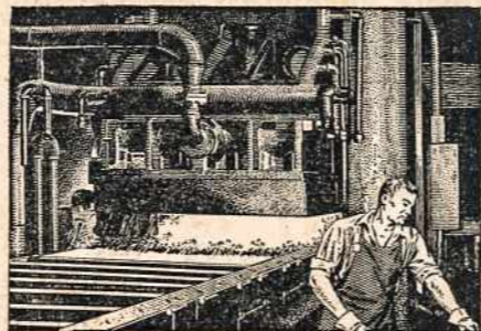
A new Ford method of quenching tank armor plate eliminates later straightening. Dies hold the plate during the process. Forty hours are saved on each M-4 medium tank and M-10 tank destroyer hull.
