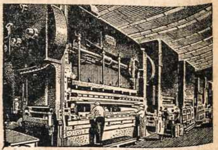
A forest of automotive-type presses speeds the production of Ford-built Liberator bombers at Willow Run. One huge press alone saves more than 100 hours building wing-tips for these planes.
