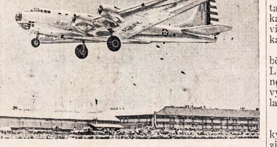
Douglas B-19 bomber, largest airplane ever built, is pictured above as it took off on its first test hop from Clover field, Santa Monica, Calif. The mighty plane lifted from the concrete runway amid a rousing cheer from Douglas workers and army officials. Army air corps ace test pilot, Stanley Umstead, was at the controls.
