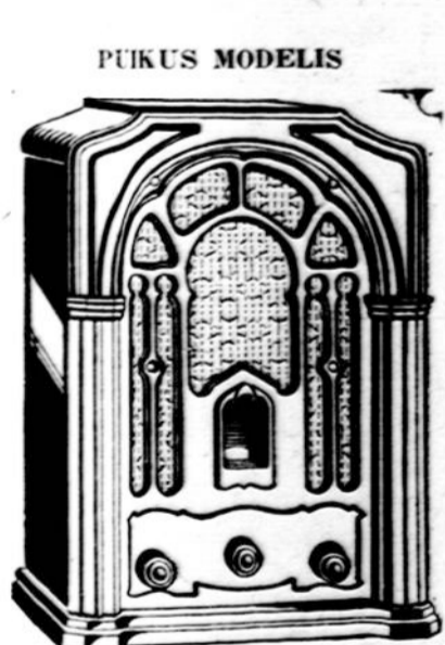
PIUKUS MODELIS Ten Tube Superheterodyne. "B" Amplification. All New Type Radiotrons. Automatic Volume Control. Tone Control. Height 29 inch.; width, 14 1/4 inch.; depth, 11 1/4 inch. Radiotrons: 4 RCA-56, 3 RCA-58, 2 RCA-65, 1 RCA-82.
