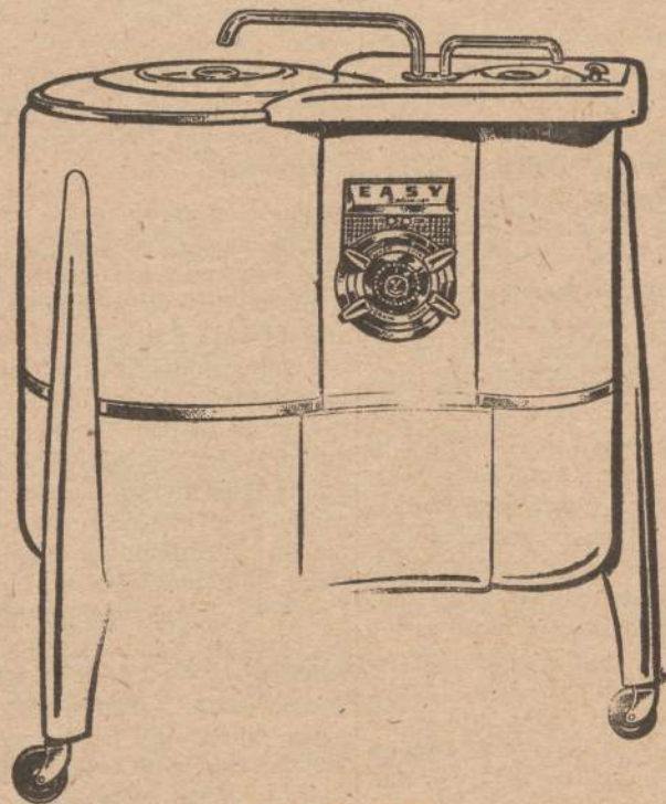
MODEL SDK
