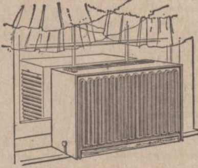
HOTPOINT MODEL ACA92 9,000 btu super-quiet Hotpoint bedroom air conditioner featuring easy, U-Mount installation; 115 volts; pushbutton "Cooling" and "Fan" settings; thermostat temperature dial has 8 settings. Exhaust air control.
